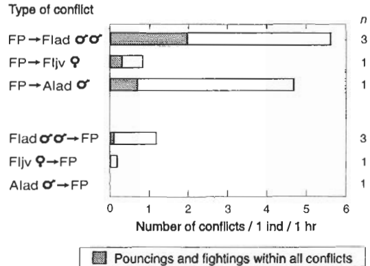
Fig. 1. Aggressiveness (mean number of conflicts initiated by 1 individual during 1 hr) between the parous female (FP) and intruders in regard to their species, sex and age. Arrows show animals active in conflicts, i.e. FP→FI means that the parous female attacked conspecific intruder, AI→FP means that N. anomalus intruder attacked the parous female, etc. n – number of 6-hr observations of a particular type of conflicts.
